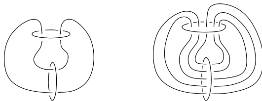
FIGURE 3. Examples of links obtained by adding crossing circles to double coil knots and untwisting.
