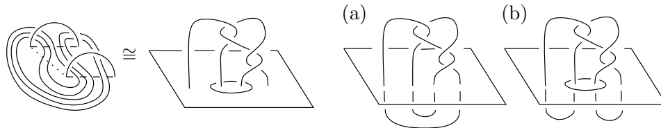
FIGURE 5. (a). Constructing the 2–bridge knot of slope 2/5 . (b). Constructing the clasped 2–bridge link of slope 2/5 .
