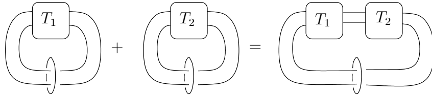
FIGURE 6. A belted sum.
