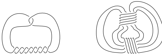
FIGURE 2. Left: a (1,2) double coil knot. Right: a (3,5) double coil knot.
