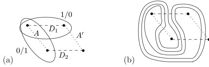
FIGURE 4. (a) A framing for the 4-punctured sphere. (b) The curve 2/5 .
