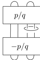
FIGURE 7. The belted sum whose complement is homeomorphic to S^3 \setminus L_{p/q} .
