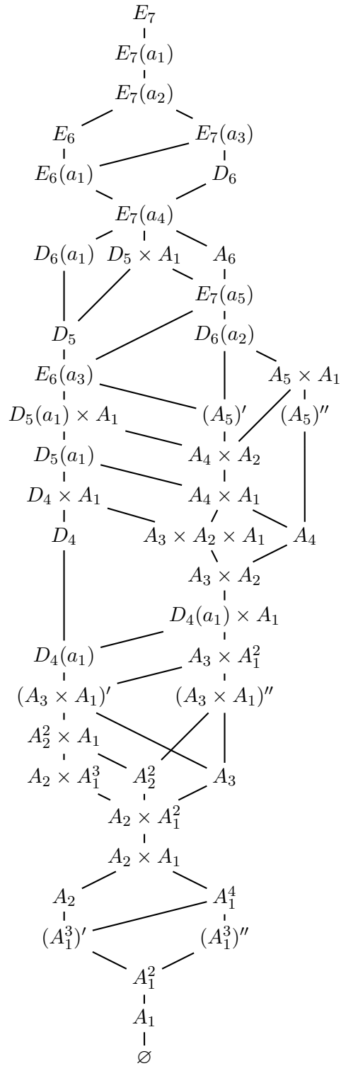
Figure 3.7: Ordering on nilpotent orbits for E_7
