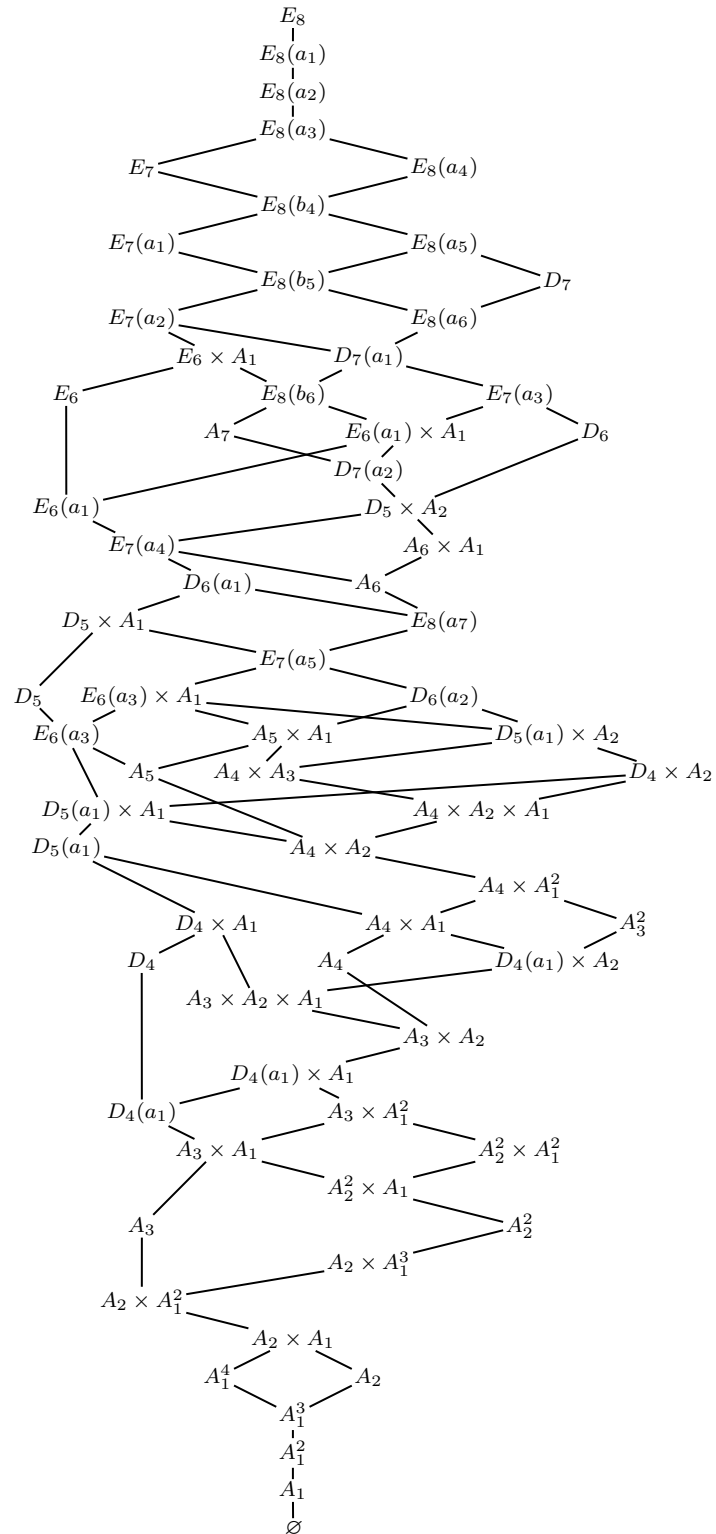
Figure 3.8: Ordering on nilpotent orbits for E_8
