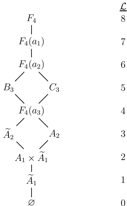
Figure 6.2: Special Orbits for F_4
