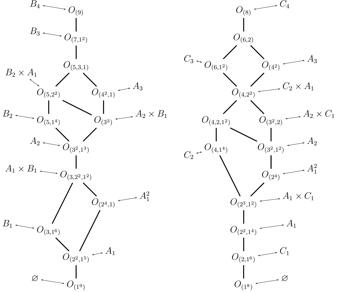
Figure 3.2: Ordering on nilpotent orbits for \mathfrak{so}_9(\mathbb{C}) (left) and \mathfrak{sp}_8(\mathbb{C}) (right)
