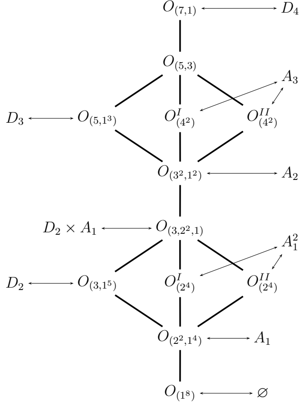
Figure 3.3: Ordering on nilpotent orbits for \mathfrak{so}_8(\mathbb{C})
