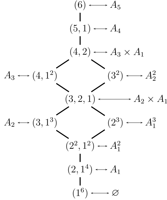
Figure 3.1: Nilpotent Orbits for \mathfrak{g} = \mathfrak{sl}_6(\mathbb{C})
