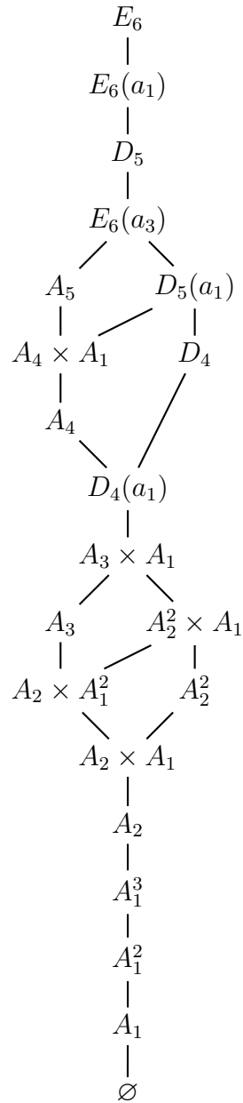
Figure 3.6: Ordering on nilpotent orbits for E_6
