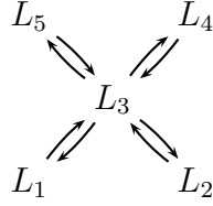
Figure 4.4: The X \text{Ext}^1 -quiver
