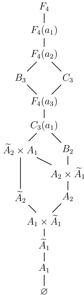
Figure 3.5: Ordering on nilpotent orbits for F_4
