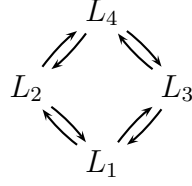
Figure 4.2: \text{Ext}^1 -Quiver of a Diamond Linkage Class
