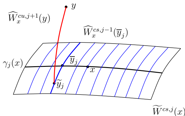
FIGURE 1. The points \tilde{y}_j and \bar{y}_j .
